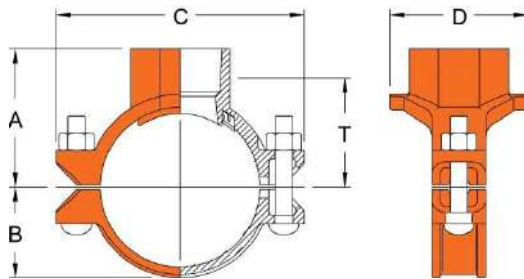
Model 7721 Mechanical Tee, Female Threaded Outlet
